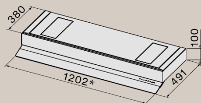
120 cm filter hood module
