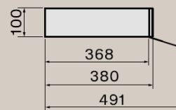
side view without front
