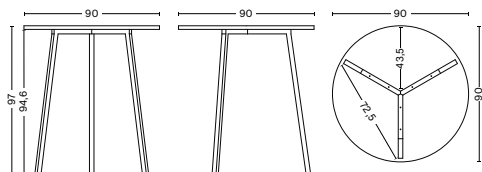
LOOP STAND HIGH ROUND | Ø90 DIAMETER 90 CM HEIGHT 97 CM TABLETOP THICKNESS 2,4 CM
