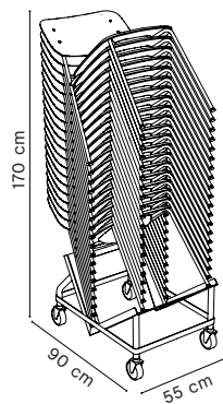
SOFT EDGE 10 Max. 20 pcs. H170 x W55 x D90 cm
