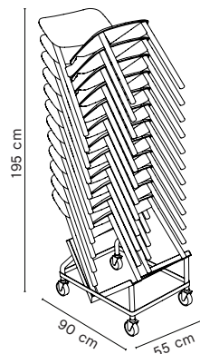
SOFT EDGE 12* Max. 12 pcs. H195 x W55 x D90 cm
