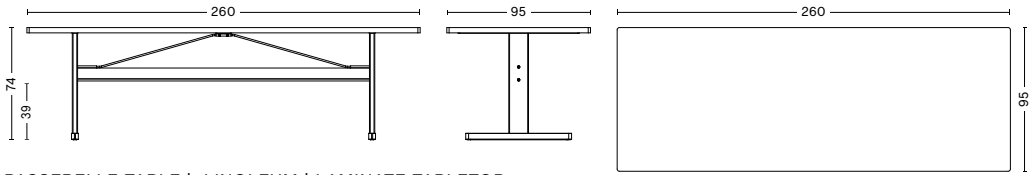
PASSERELLE TABLE | LINOLEUM | LAMINATE TABLETOP WIDTH 260 CM | 102.5" DEPTH 95 CM | 37.5" HEIGHT 74 CM | 29.25" CROSSBAR HEIGHT 39 CM | 15.5"
