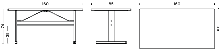
PASSERELLE TABLE | LINOLEUM | LAMINATE TABLETOP WIDTH 160 CM | 63" DEPTH 85 CM | 33.5" HEIGHT 74 CM | 29.25" CROSSBAR HEIGHT 39 CM | 15.5"
