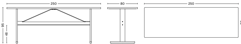
PASSERELLE HIGH TABLE | LINOLEUM | LAMINATE TABLETOP WIDTH 250 CM | 98.5" DEPTH 80 CM | 31.5" HEIGHT 95 CM | 37.5" CROSSBAR HEIGHT 48 CM | 19"
