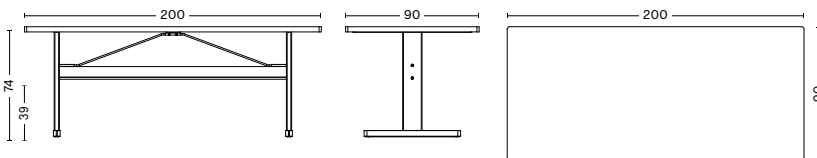
PASSERELLE TABLE | LINOLEUM | LAMINATE TABLETOP WIDTH 200 CM | 78.75" DEPTH 90 CM | 35.5" HEIGHT 74 CM | 29.25" CROSSBAR HEIGHT 39 CM | 15.5"
