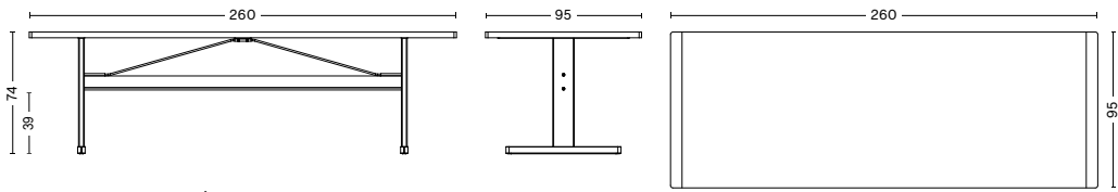
PASSERELLE TABLE | VENEER TABLETOP WIDTH 260 CM | 102.5" DEPTH 95 CM | 37.5" HEIGHT 74 CM | 29.25" CROSSBAR HEIGHT 39 CM | 15.5"
