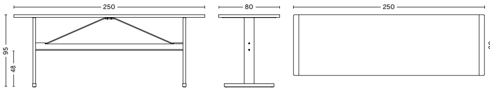
PASSERELLE HIGH TABLE | VENEER TABLETOP WIDTH 250 CM | 98.5" DEPTH 80 CM | 31.5" HEIGHT 95 CM | 37.5" CROSSBAR HEIGHT 48 CM | 19"
