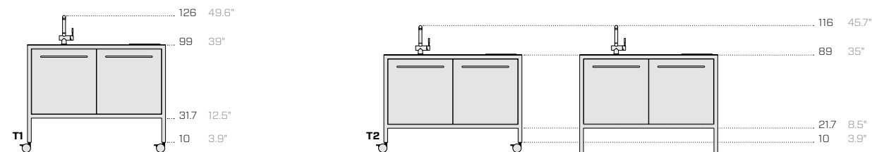
Kitchen height (with wheels) Altezza cucina (con ruote) Küchenhöhe (mit Rädern)
