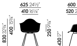
Eames Fiberglass Armchair DAX
