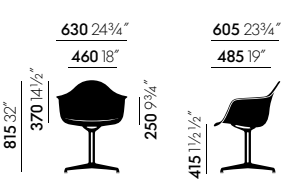
Eames Plastic Side Chair RE DAR
